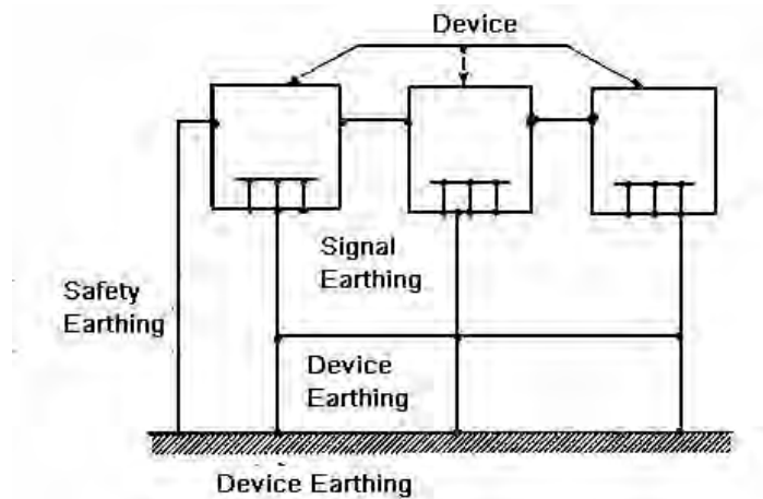
Appendix Figure 7-2 Multiple-point ground
