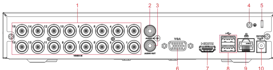
Figure 3-19 Rear panel
