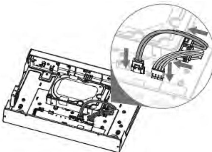
Figure 2-27 Connect cables
