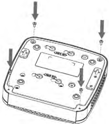
Figure 2-35 Fasten screws
