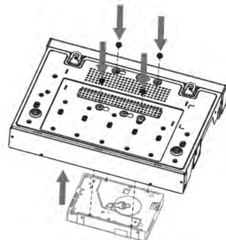
Figure 2-26 Fasten screws
