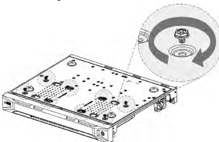
Figure 2-4 Fasten screws
