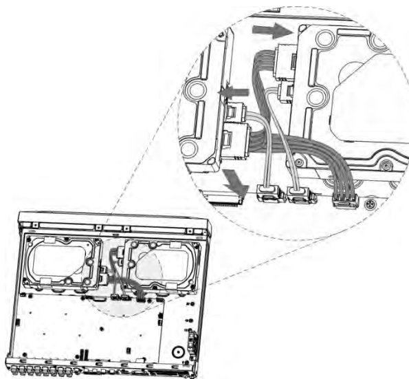
Figure 2-5 Connect cables
