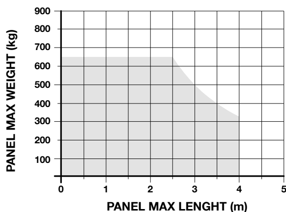
GRAPH 1 (mod. LFAB4024 / LFAB4000)
