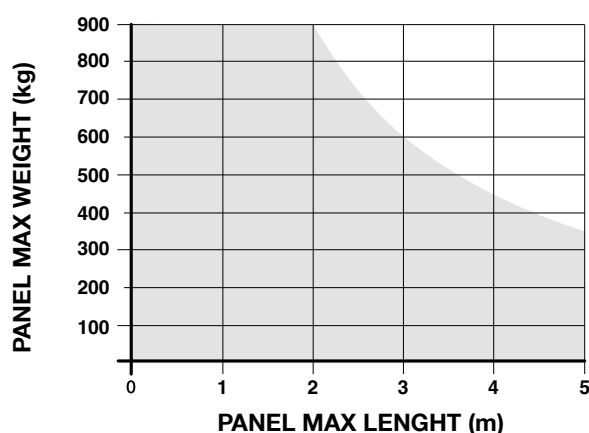
GRAPH 1 (mod. BFAB5024)
