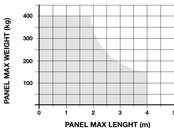
GRAPH 1 (mod. LFAB4024HS)
