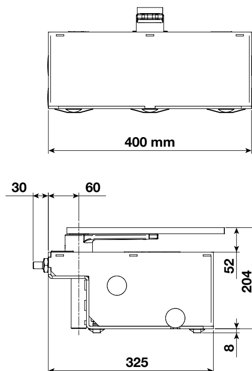
GRAPH 1 (mod. LFAB4024HS)
