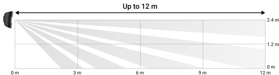
The vertical viewing angle of the detector
